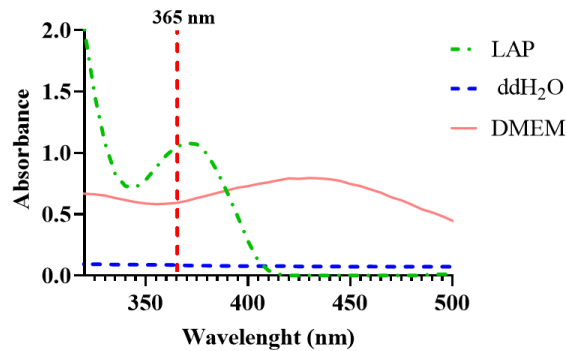
Fig 2 Evaluation of the spectra of the solution of photoinitiator (LAP) dissolved in DMEM at the concentration of 2.5 mg/mL and of the two ETD 2020 NF formulations in ddH 2 O or DMEM at the concentration of 0.5 % w/v and 1.2 % w/v respectively.
