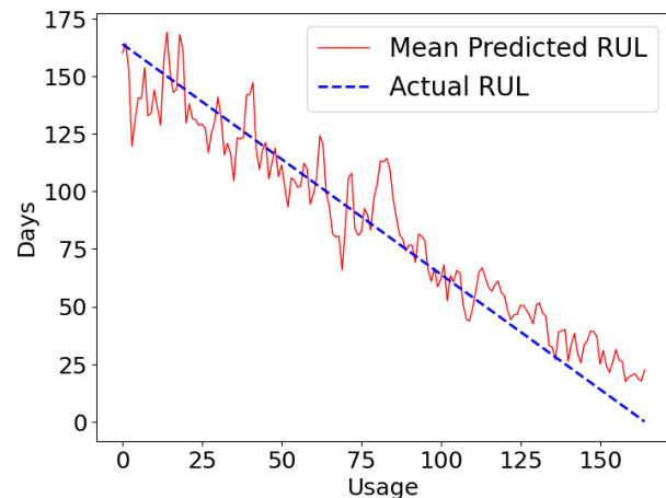
Figure 6. Case 2 - RUL estimation, WT07.
