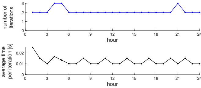
Fig. 6. Winter period: number of iterations and average time per iteration for the optimisation with variable efficiencies.
