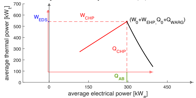
Fig. 21. Graphical representation of the maximum upward flexibility condition on the electrical side at hour 10 am.
