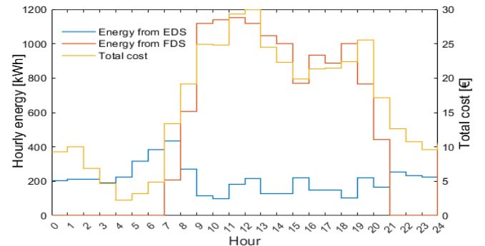
Fig. 16. Optimal cost and related electricity and fuel absorbed during the day.
