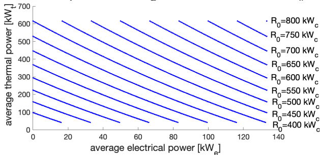
Fig. 18. Electrical input from the EHP and thermal input from the WARG to supply the cooling demand.
