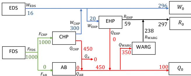
Fig. 19. Solution of the optimisation with variable efficiencies at hour 10 am.
