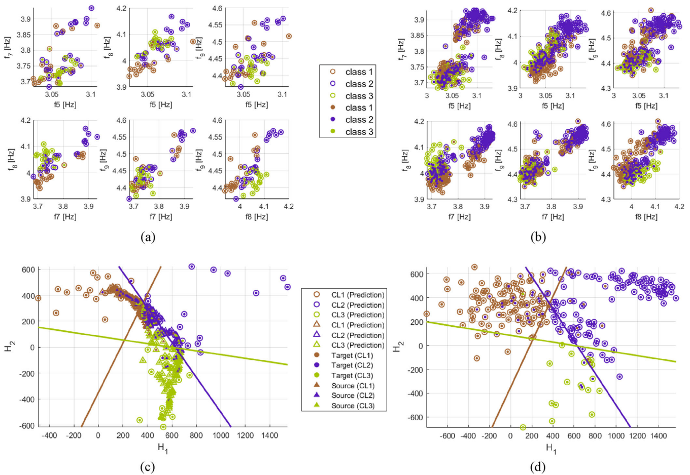
FIGURE 15 (a) SVM model obtained providing a training data set consisting of only 54 observations obtained for Church of Santa Caterina (projections of the four-dimensional space); (b) testing of SVM model; (c) training phase of kernelized Bayesian transfer learning (KBTL) model, trained on 54 observations of the Church of Santa Caterina (circle) and on 300 observations of the Sanctuary of Vicoforte (triangle); and (d) testing of the KBTL model.
