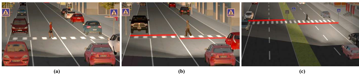
Fig. 2. Crosswalks (a) without, (b) with fixed LED strips and road section with one lane per direction, and (c) with fixed LED strips and road section with two lanes per direction. In the fixed LED condition, the pedestrian crossed the road with the led bar always on. In the flashing condition, the bar operated with a flashing light at a frequency of 2 Hz. The light was activated when the pedestrian stepped inside an area monitored by a set of virtual cameras.
