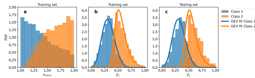
Figure 9. One dimensional example: (a) PDFs over binned data of the training set for the two classes ( \overline{Nu} < 500 and \overline{Nu} \geq 500 ) reported against the normalized flow velocity. (b) PDFs over binned data of the training set for the two classes reported against the mixed feature y_1 , constructed according to Equation (13) and choosing the point of the Pareto front with the least overlapping of the two classes according to the Bhattacharyya distance, along with a GEV analytical fitting of the two binnings. (c) PDFs over binned data of the testing set for the two classes reported against the same mixed feature y_1 together with the same GEV fittings of the (b) subfigure. The mixed variable \tilde{y}_1 shown here is referred exclusively to this Gnielinski one dimensional optimization.
