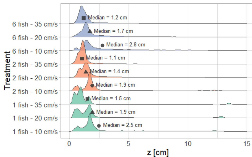
Figure 4. Vertical probability density ( P_V ) for different group sizes and velocities (bottom of the flume: z=0 ; free water surface: z=15 cm). Each P_V is retrieved with Kernel density estimation of all vertical fish positions detected at the respective flow velocity and group size.
