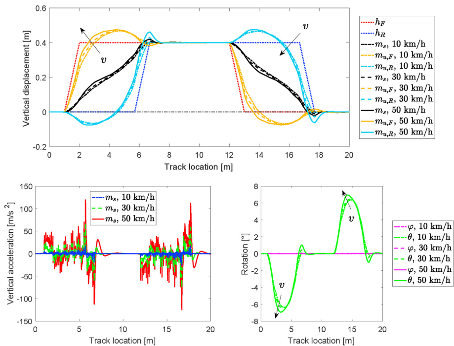
Fig. 23. Longitudinal speed effect on tracked vehicle CMS model: long hill track.
