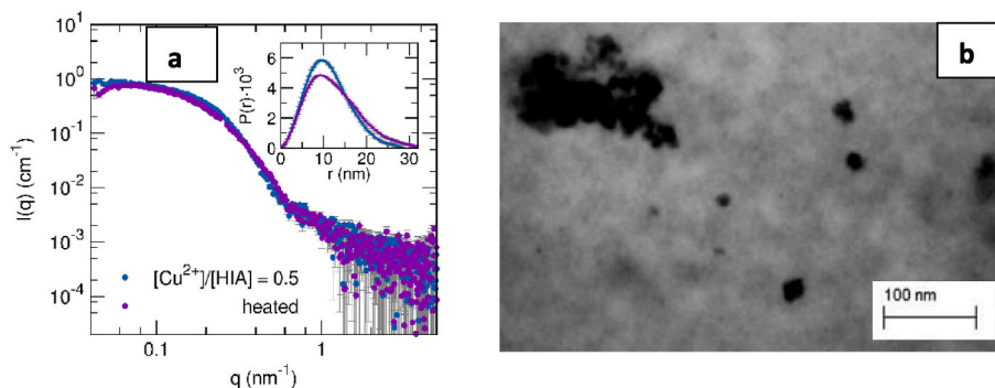
Fig. 10. a) The SAXS data of H_{38}\text{-}b\text{-}G_{475}/\text{Cu}(\text{OAc})_2 ([HIA] = 1.8 mM) with [\text{Cu}^{2+}]/[\text{HIA}] = 0.5 collected at 25^\circ \text{C} before (blue dots) and after (purple dots) a heating cycle up to 65^\circ \text{C} . In the inset, the corresponding pair distance distribution functions are reported; b) STEM images without contrast agent of \text{Cu}(\text{OAc})_2/H_{38}\text{-}b\text{-}G_{475} PIM micelles ([HIA] = 1.8 mM; [\text{Cu}^{2+}]/[\text{HIA}] = 0.5 ) taken at 25^\circ \text{C} after heating to 65^\circ \text{C} . (For interpretation of the references to color in this figure legend, the reader is referred to the Web version of this article.)
