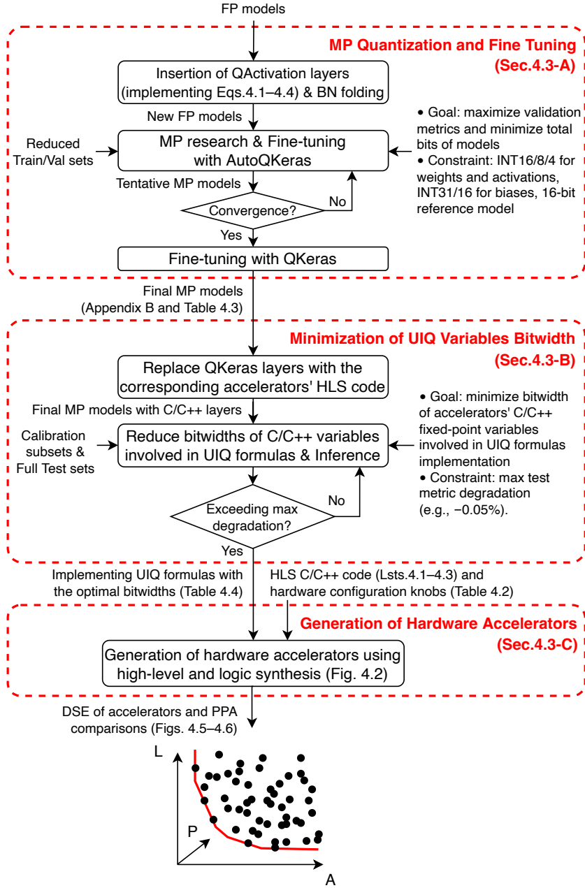
Figure 4.4: Accelerators design flow. Image taken from [28].
