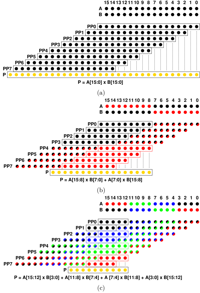
Figure 3.8: Alignment of PPi partial products for CONFIG 16 \times 16 / 16 \times 8 (a), 8 \times 8 / 8 \times 4 (b) and 4 \times 4 (c). Images taken from [26].
