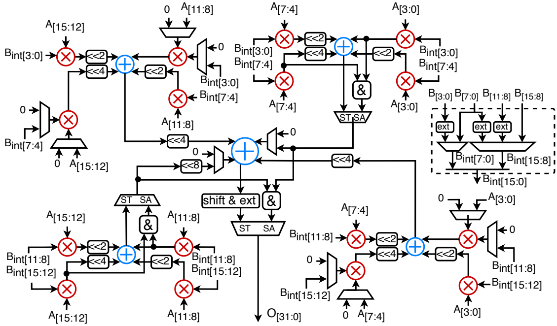
Figure 5.4: The proposed STAR D&amp;C architecture. Image taken from [27].
