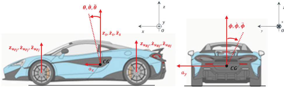
Figure 3. Lateral and rear views of a vehicle, showing the main variables considered in the computation of the objective metrics: (i) heave ( z_s, \dot{z}_s, \ddot{z}_s ), roll ( \phi, \dot{\phi}, \ddot{\phi} ) and pitch ( \theta, \dot{\theta}, \ddot{\theta} ) displacements, speeds, and accelerations of the sprung mass; (ii) longitudinal and lateral accelerations of the vehicle ( a_x, a_y ); and (iii) vertical displacements, speeds and accelerations ( z_{u_{ij}}, \dot{z}_{u_{ij}}, \ddot{z}_{u_{ij}} ) of the unsprung masses of the four corners, where the subscript i = F, R indicates the front or rear axles, and the subscript j = L, R the left or right vehicle sides.
