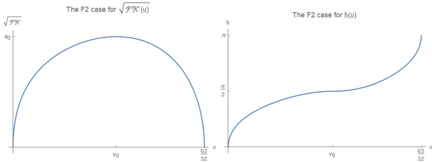
Fig. 10 On the left the plot of the function \sqrt{\mathcal{FK}^{\mathbb{F}_2}(v)} corresponding to \alpha = 1 and explicitly displayed in Eq. (7.4). On the right the corresponding function h(v) providing the homeomorphism to the right ascension angle
