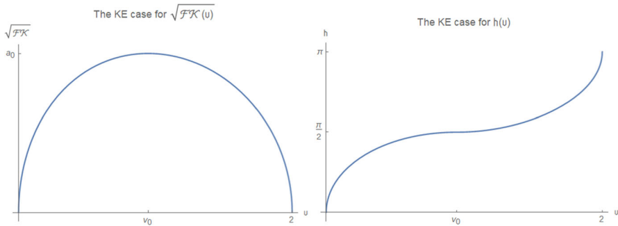
Fig. 11 On the left the plot of the function \sqrt{\mathcal{FK}^{KE}(v)} corresponding to \lambda_1 = 1, \lambda_2 = 2 and explicitly displayed in Eq. (7.5). On the right the corresponding function h(v) providing the homeomorphism to the right ascension angle
