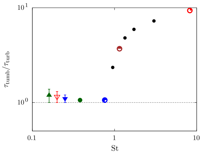
FIG. 2. Ratio between the fiber tumbling time [evaluated from Eq. (3)] and the eddy turnover time at the fiber length scale [evaluated from Eq. (7)] as a function of the Stokes number. Colored bullets refer to the simulation data, while colored triangles are the experimental data. Coloring and symbols correspond to the values of St used also in the following figures.
