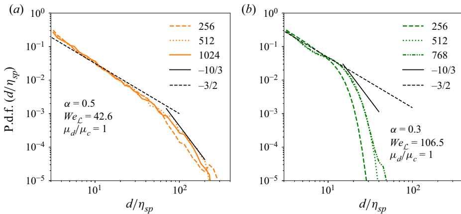
Figure 26. Effects of grid size on the DSD for (a) cases Cx4 at \alpha = 0.5 , \mu_d/\mu_c = 1 and We_{\mathcal{L}} = 42.6 , panel, and (b) cases Wx3 at \alpha = 0.3 , \mu_d/\mu_c = 1 and We_{\mathcal{L}} = 106.5 . Blacklines represent the -3/2 (dashed) and -10/3 (continuous) power-law scalings.
