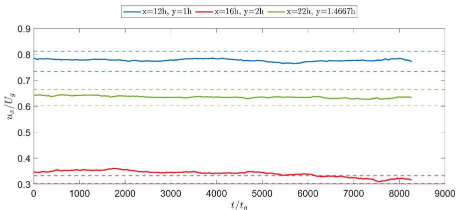
Fig. 3. Running average of streamwise velocity, u_x , at different points in the spanwise plane ( z/h = 1 ) with window size of 0.2 s ( 4300 t_g ). The horizontal axis shows the normalized time from the beginning of the simulation.
