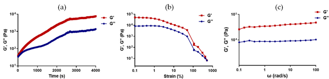
Figure 3. Rheological analysis of CHAF_1 sample. (a) Time sweep. (b) Strain sweep. (c) Amplitude sweep.
