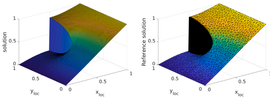
Fig. 12. test3: Slice plot of the solution with the proposed approach (left) and reference solution (right).
