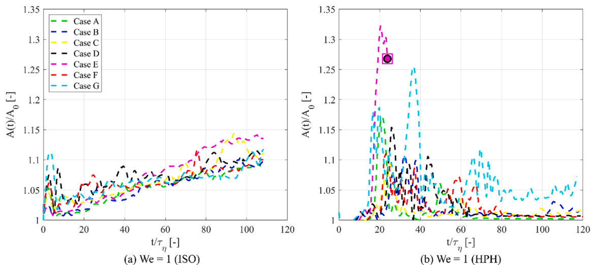
Fig. 14. Total interfacial area, A , as a function of time, t , for the cases of ISO (a) and HPH (b) at We=1 . Hollow square marks the state of initial breakup and solid disc marks the state of first effective breakup.
