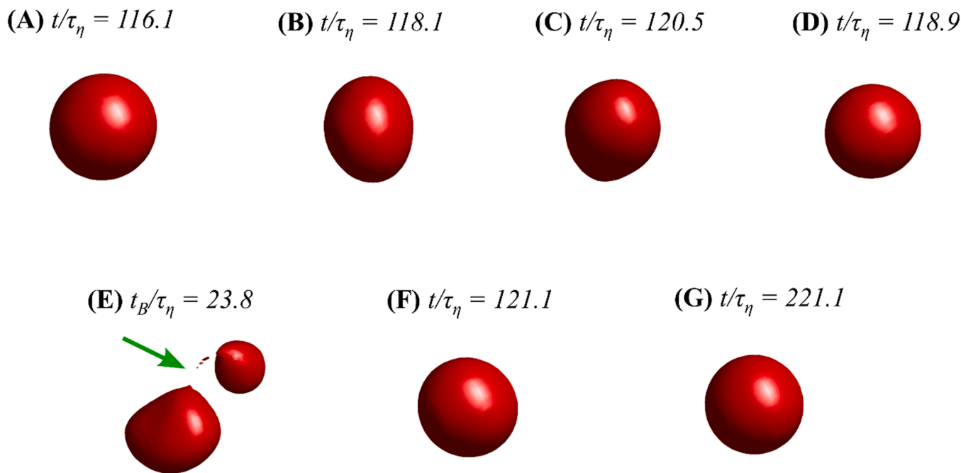
Fig. 13. Deformation morphology of drops for case HPH at the instance of first effective breakup showing drops A-G at We=1 . (Iso-surfaces of VOF=0.5 ). The final simulation times normalized with the Kolmogorov timescale are specified for each case. For case E where breakup occurs, the normalized first effective breakup time is specified. Green arrow shows the position of first effective breakup. (For interpretation of the references to colour in this figure legend, the reader is referred to the web version of this article.)
