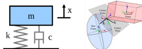
Figure 7 Ground contact force model (left) and Simscape model (right).
