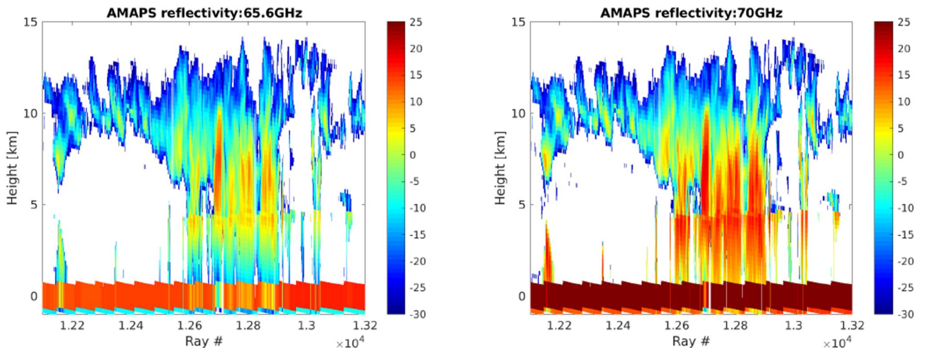
Figure 14. Simulation of reflectivities (with colorbar values in dBZ) for an AMAPS radar with frequency at 65.6 and 70 GHz in correspondence to the scene shown in Figure 13. A pulse width of 3.3 \mu\text{s} is assumed.
