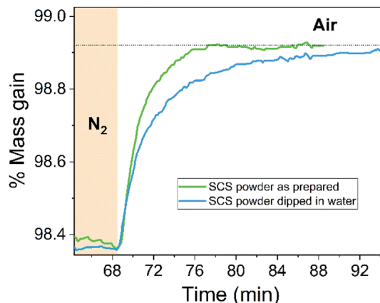
Fig. 9 TGA analysis comparison between SCS powder as synthesized and after being dipped in water and dried. Only the oxygenation step after reduction is shown. TGA temperature was maintained at 480 °C during the redox process.
