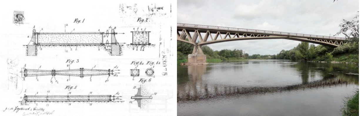
Figure 1 (a) Italian patent n.2830875 by E. Freyssinet and J. Séailles: Processo di prefabbricazione di reinforced concrete, October 1929 (Courtesy of Archivio Centrale dello Stato); (b) Concrete Arch bridge of Châtel-de-Neuvre by E. Freyssinet (Courtesy of www.freyssinet.com ).
