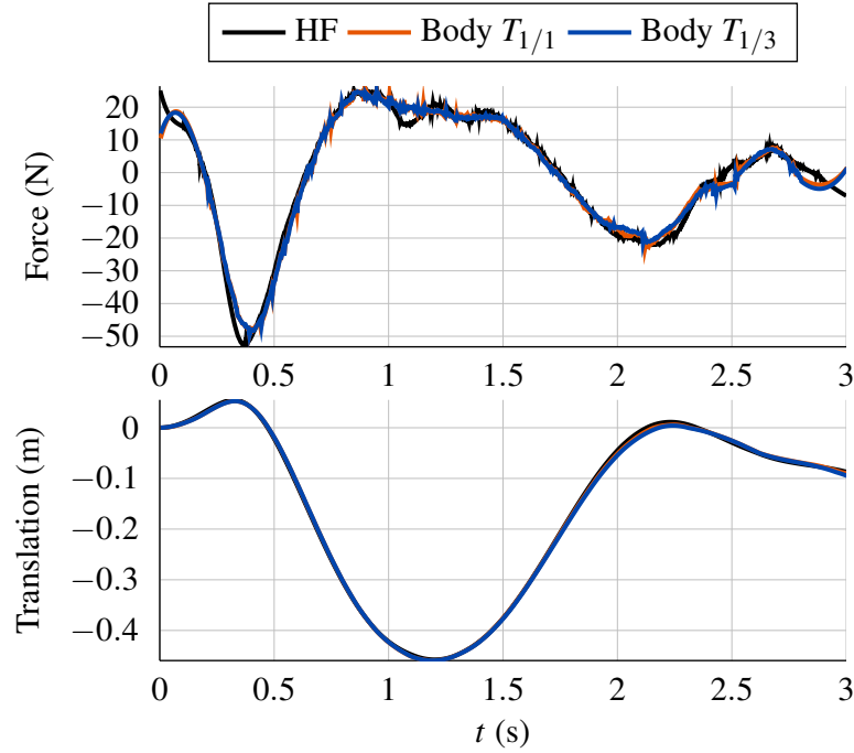
Fig. 4.26 Evolution of the force acting on the body and the heave motion of the body over time. The solutions from the coupled model are compared to the high-fidelity simulation solution over \Omega_{HF} used to build the basis functions (HF).
