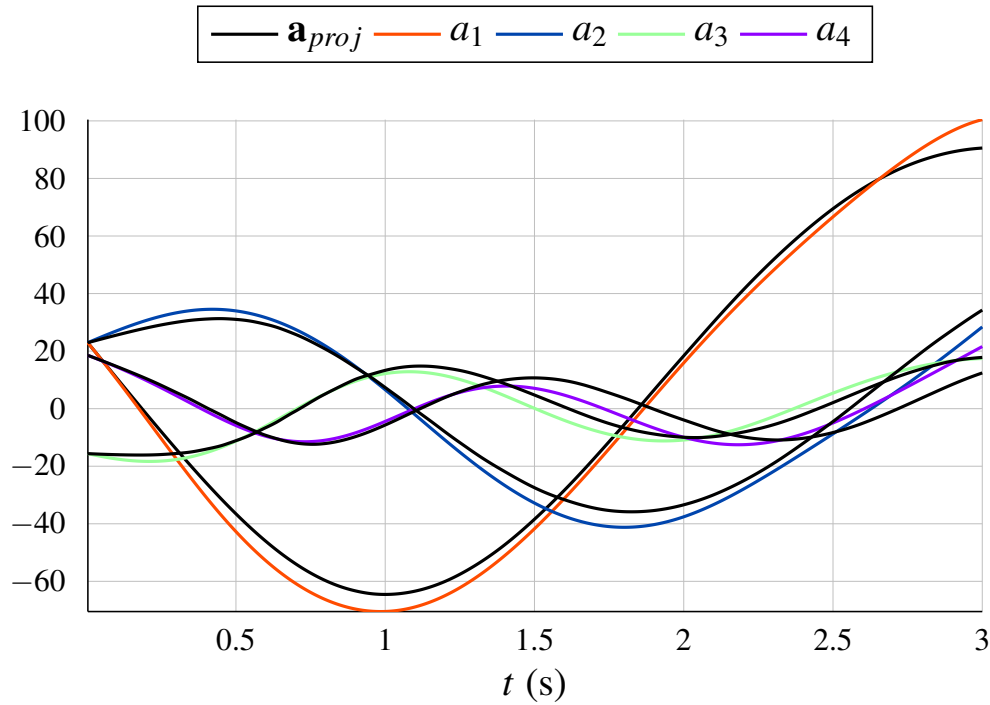
Fig. 3.30 Evolution of the first four temporal coefficients (in color) for case R_p = 2 , compared to their respective projection coefficients (in black).
