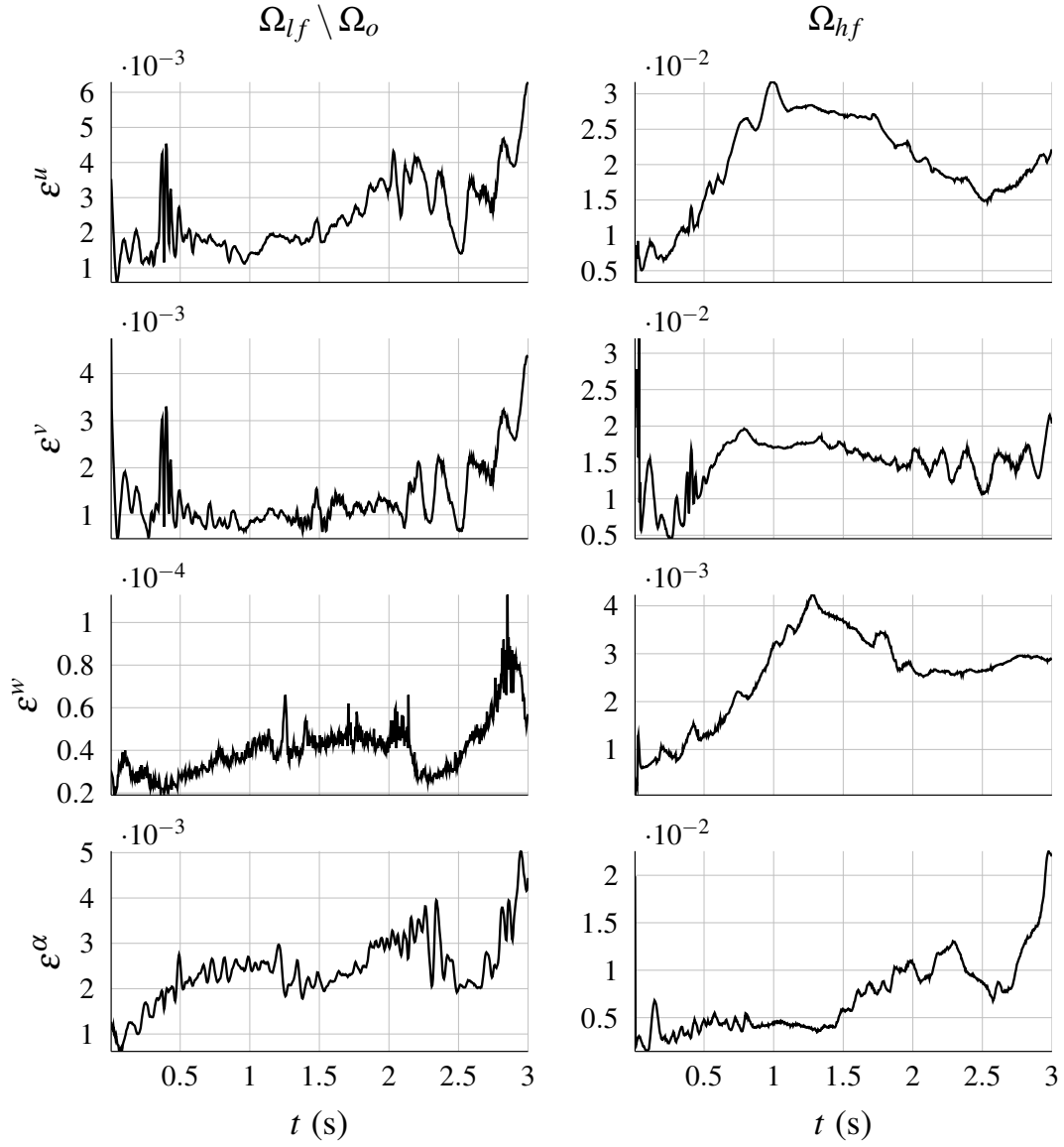
Fig. 4.15 Evolution of the absolute errors for the velocity and VOF fields over time, over the high-fidelity domain \Omega_{hf} and over the remaining low-fidelity domain \Omega_{lf} \setminus \Omega_o . The POD ROM model is built with N_r = 30 and N_s = 750 .
