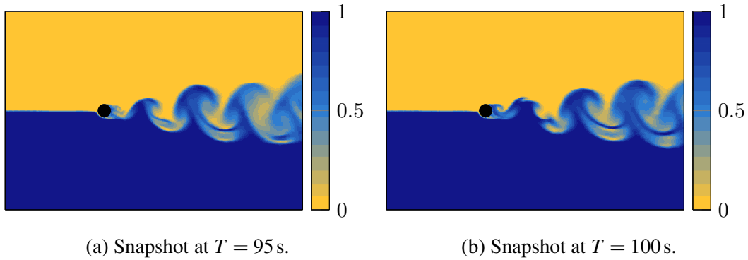
Fig. 3.19 Snapshots of the VOF field on a x - y section for the cylinder in the biphasic flow with same density and different dynamic viscosity (case LoRe ).
