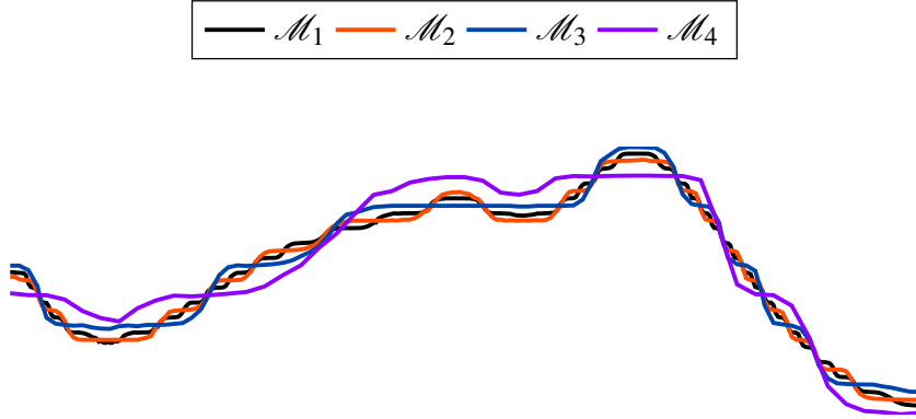
Fig. 4.7 Outline of the free surface (located at \alpha = 0.5 ), for the different mesh discretizations \mathcal{M}_i .
