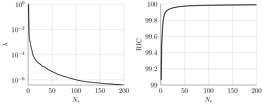
Fig. 3.34 Evolution of the eigenvalues spectrum, normalized to the first eigenvalue (left), and of the RIC (right) with respect to the number of DMD modes N_r . The plots show only the first 200 modes.
