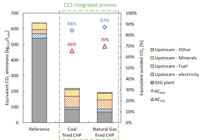
Fig. 3. Detail on the equivalent CO 2 emissions with and without CCS integration.
