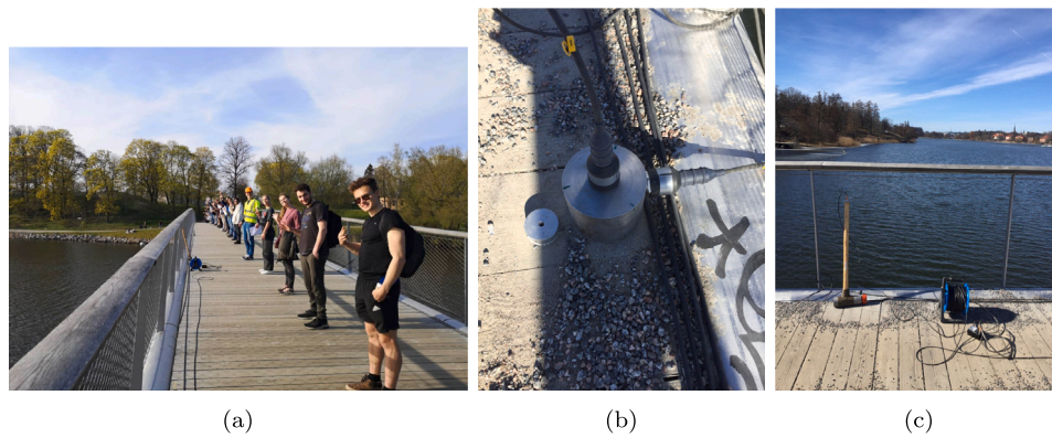
Fig. 4. Photographs from the in situ survey on day two: (a) Pedestrians in position for the loaded case. (b) One of the accelerometers.
