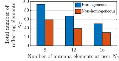
Figure 3: Average number of reflecting elements \bar{N}_T aiding AP to user communication when tags are distributed homogeneously and non-homogeneously with \lambda = 2 and N_T = 8 .
