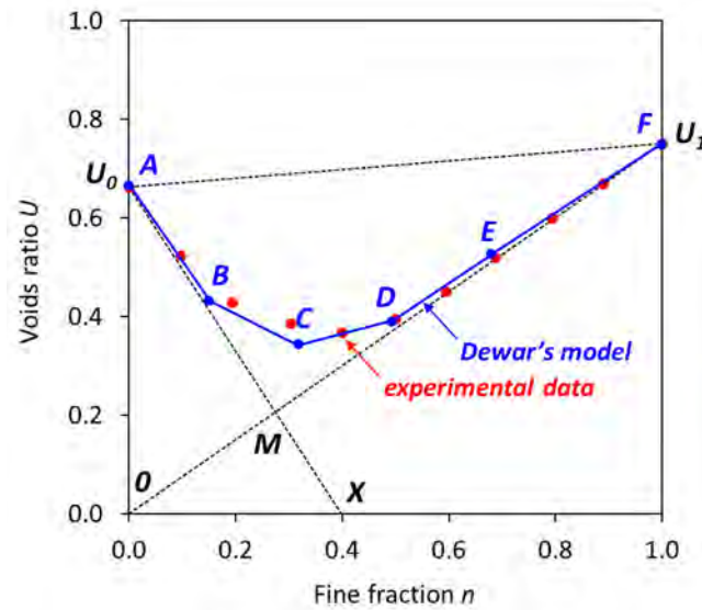
Figure 1. Theoretical voids ratio diagram.
