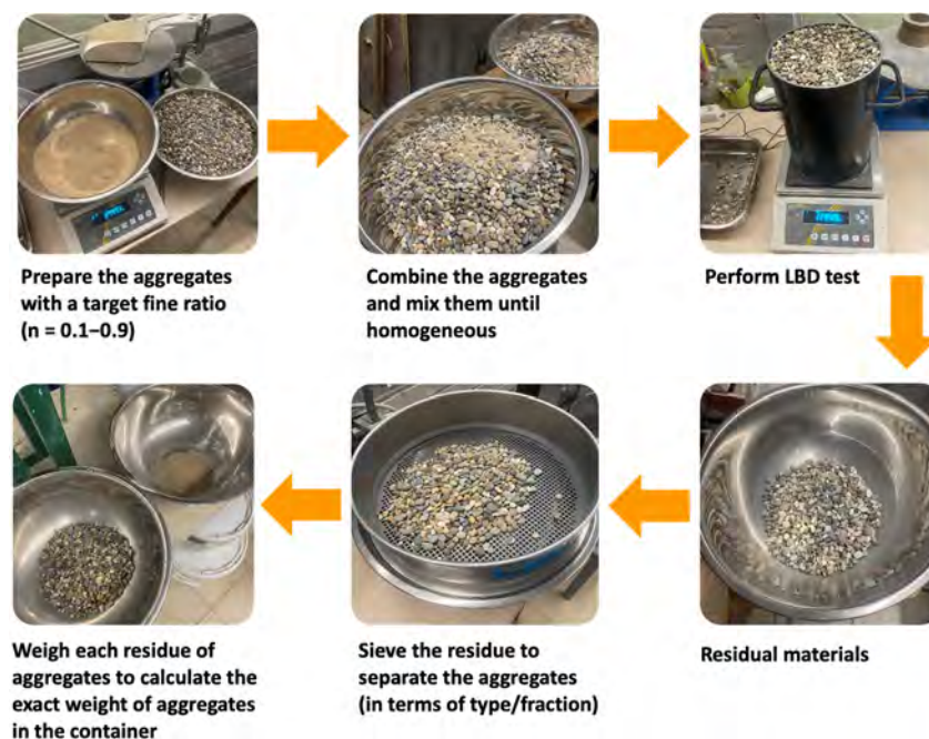
Figure 5. Schematic procedure of the LBD test on aggregate mixtures.
