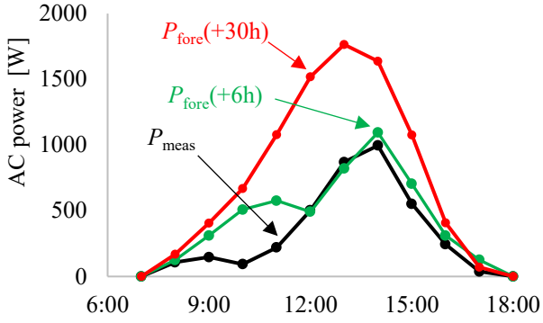
Fig. 4. Progressive improvement in the AC power predictions for a cloudy day (6 th Feb 2022).
