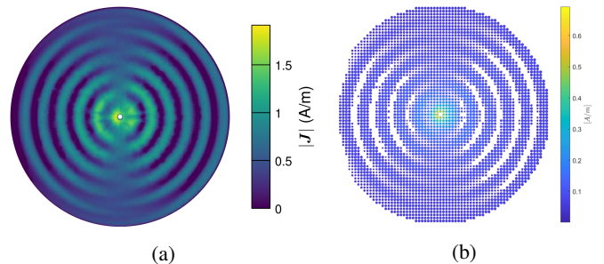
Fig. 2: Circular MTS antenna with linear pol. broadside radiation: (a) Optimized surface current profile, (b) simulated surface current with unit-cell implementation.
