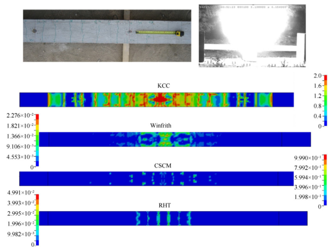
Fig. 5. On the top, field test photo corresponds with the bottom part of the beam B2 tested and high-speed video frame of the detonation. Bottom view of the beam models corresponding to the 15 mm meshes. Legends show the effective plastic strain of the concrete model of the beam.
