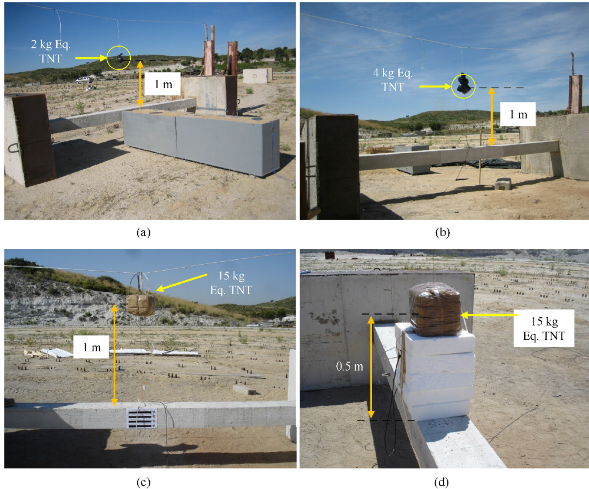
Fig. 1. Images of the experimental field campaign: (a) Beam B1 (same settings as B2 and B3); (b) Beam B4; (c) Beam B5; (d) Beam B6.
