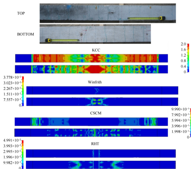
Fig. 8. Field test photos correspond with the top and bottom part of the beam B4 tested. Top and bottom view of the beam models corresponding to the 20 mm meshes. Legends show the effective plastic strain of the concrete model of the beam.
