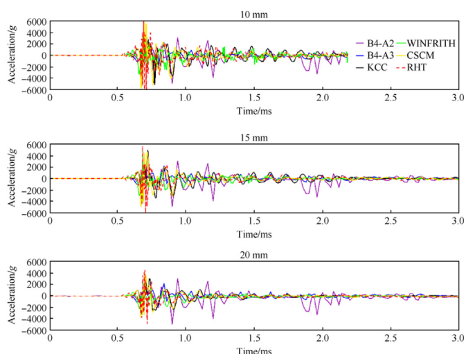
Fig. 7. Acceleration values corresponding to the locations A2/A3 in test B4 showing the differences between concrete models (see Table 4).
