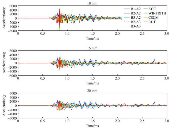
Fig. 4. Acceleration values corresponding to the locations A2/A3 in tests B1, B2 and B3 showing the differences between concrete models (see Table 3).
