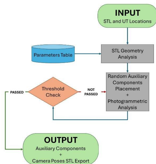
Figure 2. Methodological pipeline
