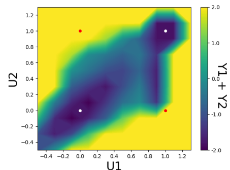
(c) Decision boundary for XOR operation
