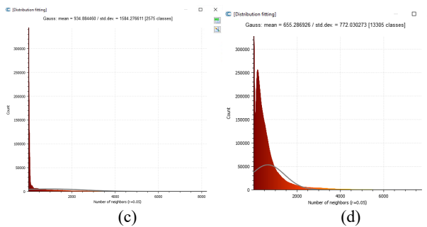
Figure 4. Points quality distribution using the density analysis, normalization 0-90 in the colour ramp for improving visualization): (a) dynamic acquisition dataset and (b) the static acquisition, (c) and (d) the respective gaussian distribution
