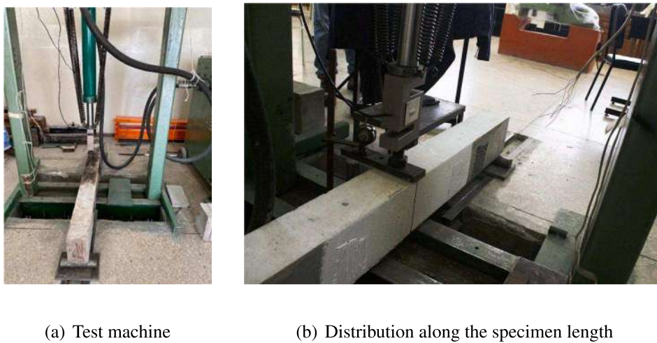
Fig. 8. Test setup and instrumentation.
