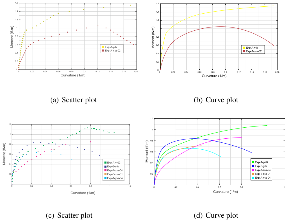
Fig. 21. Analytical moment–curvature diagram.
