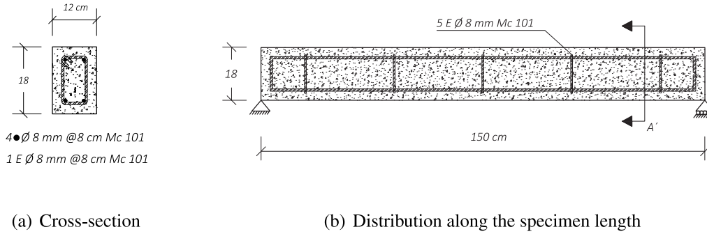
Fig. 2. Steel reinforcement details of specimens.
