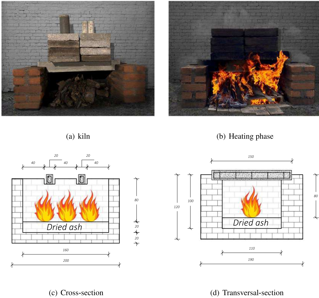
Fig. 7. Heating phase.
