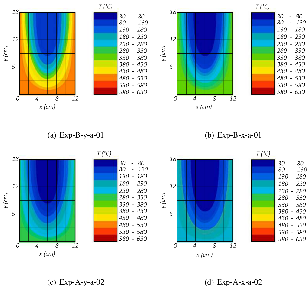
Fig. 14. Temperature distribution.
