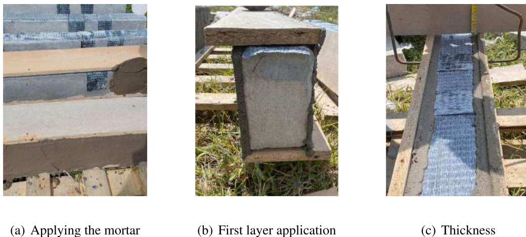
Fig. 5. Installing mortar insulation jackets.
