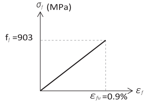
Fig. 12. Stress-strain diagram for FRP [35].
