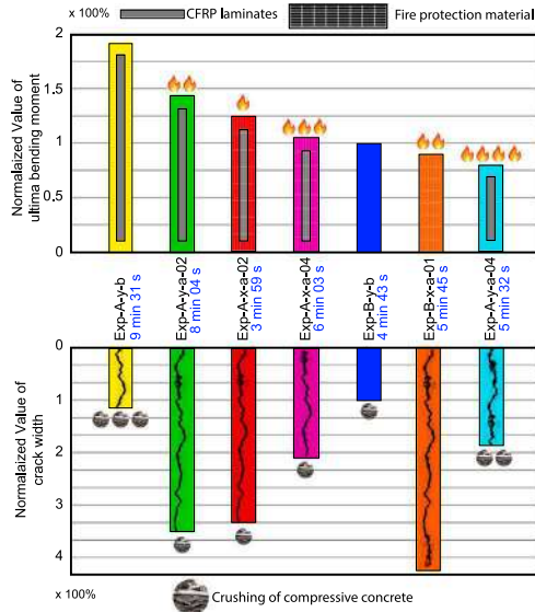
Fig. 17. Ultimated bending moment and width crack normalization.
