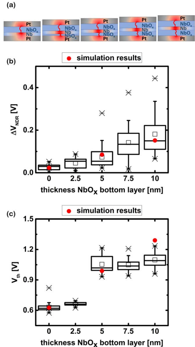
Figure 4. (a) Schematic of the five different sample stacks under investigation. Boxplots showing the distribution of (b) the voltage extension of the NDR region and (c) the threshold voltage of the five samples with different \text{NbO}_x bottom layer thicknesses for 30 measurements, respectively. The red dots in figures 4(b) and (c) represent the simulation results depicted in figure 1(b).
