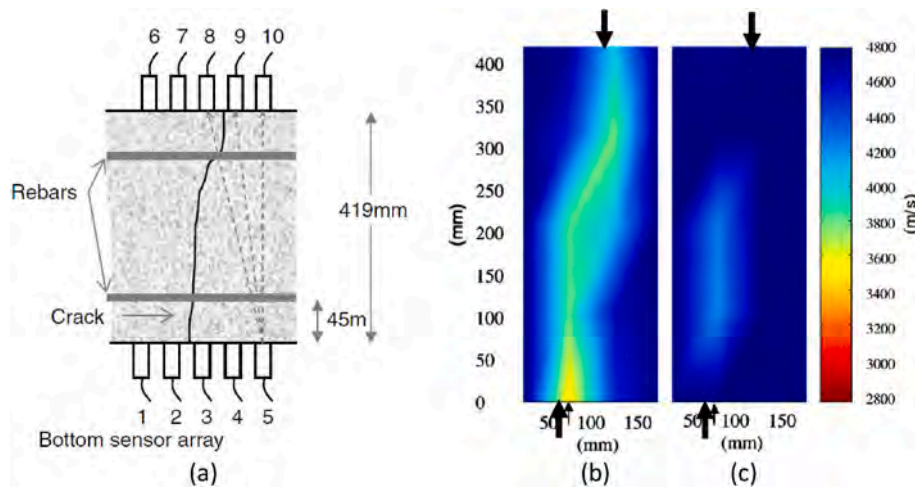
Fig. 2. (a) Side view of the sensor locations and crack position through the bridge deck, (b) ultrasonic tomogram before repair, and (c) after repair with epoxy injection in the crack (Aggelis and Shiotani, 2007).
