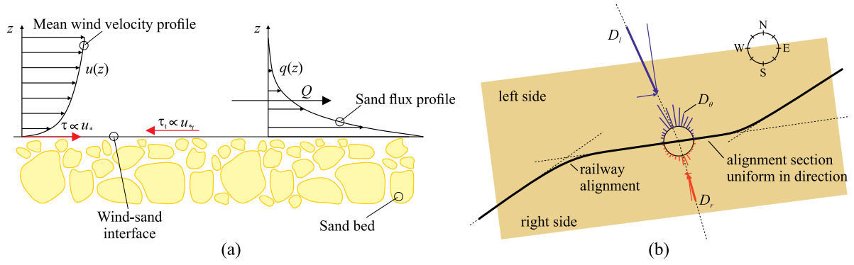
Fig. 2. Wind velocity and sand flux profiles during saltation (a), incoming left-side D_l and right-side D_r sand drift along a generic infrastructure alignment (b).
