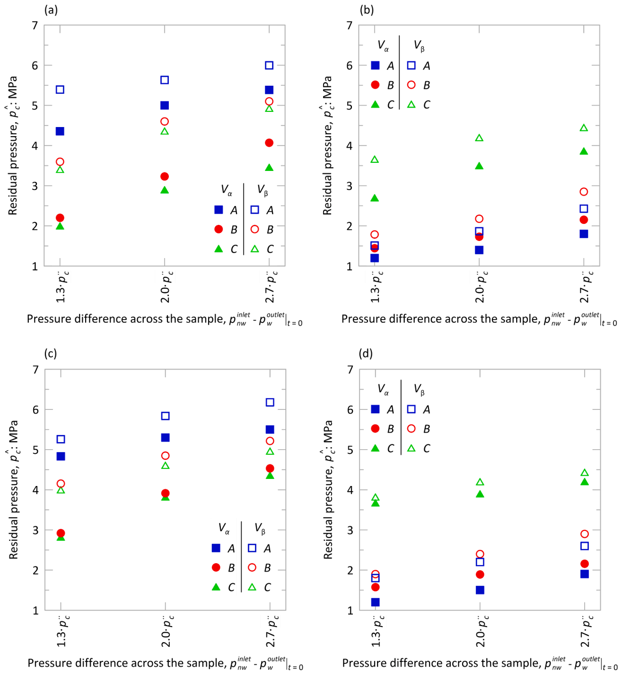
Fig. 17. Abacus of residual capillary pressure \hat{p}_c^{\delta} for all the materials, the inlet pressures, (a) the Brooks and Corey permeability and holding time equal to zero \tau_t , (b) the van Genuchten permeability and holding time equal to zero \tau_t , (c) the Brooks and Corey permeability and holding time equal to 6 h \tau_{II} , (d) the van Genuchten permeability and holding time equal to 6 h \tau_{II} with procedure II (residual method)
