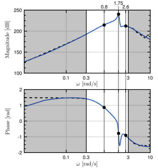
Fig. 7 Bode diagram of the radiation kernel frequency response computed with the coefficients obtained from NEMOH (dashed-black) and the moment-matching parametric model frequency response (solid-blue), for three interpolation points (black dots).
