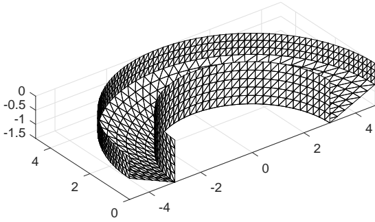
Fig. 1 The low-order mesh for the float of the OPT device
