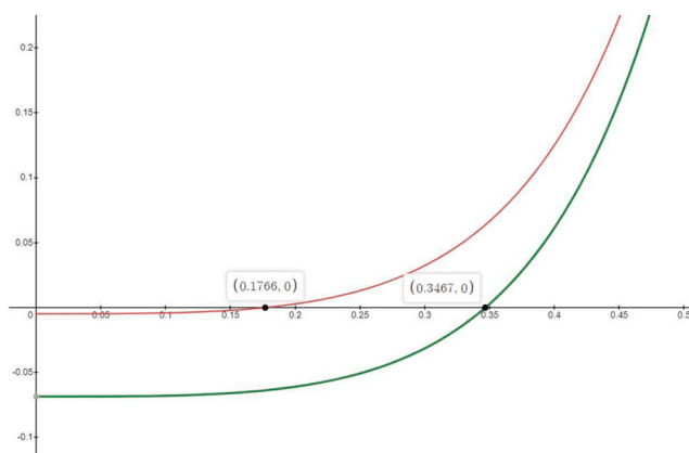
Fig. 7. Graphical solution of Eq. 4, assessed by experimental values of intrinsic Darcian permeability k_D , average pore diameter D_{av} and pore sphericity \phi .
