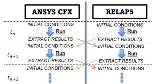
Figure 11. Explicit numerical scheme
