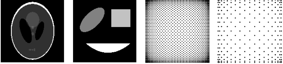
Fig. 1: The Shepp-Logan phantom (left), a geometric phantom (middle, left), as well as the Lissajous nodes \mathbf{LS}_2^{(32,33)} (middle, right) and \mathbf{LS}_2^{(10,11)} (right).
