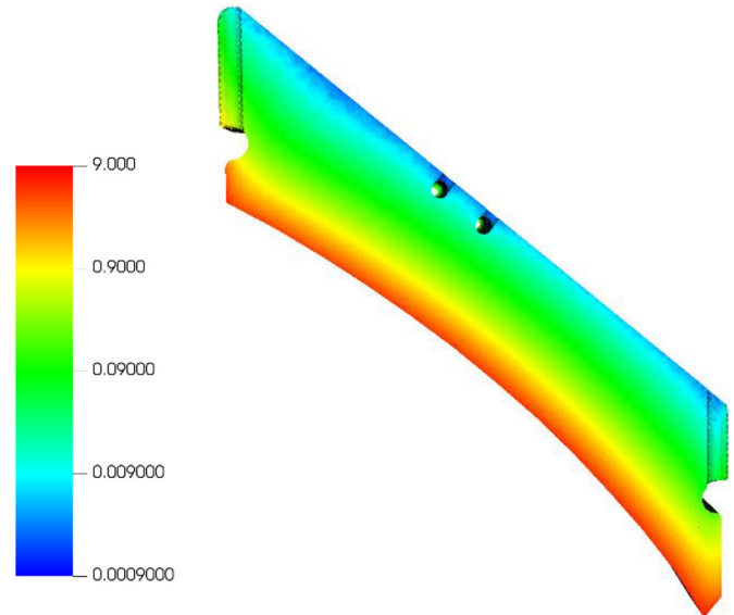
Fig. 13. DPA (in units of DPA/FPY) calculated in the EUROFER SB of the UL.
