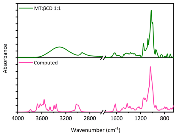
Fig. 10 FTIR experimental (green) and computed (magenta) spectra of the MT:β-CD 1:1 inclusion complex.
