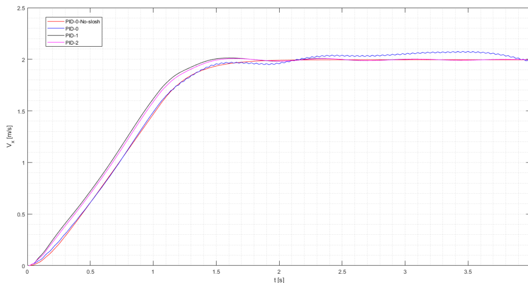
Figure 13. Comparative response between sloshing and non-sloshing simulation for different PID gain scheduling strategies.
