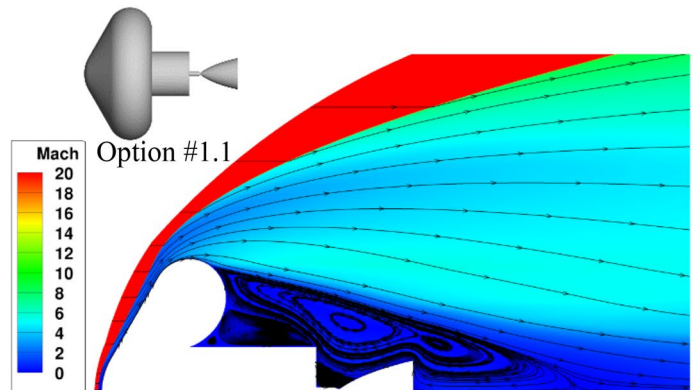
Fig. 13 Flight point under investigation for the CFD simulations for the reference shape (option #1.1) (left), flow topology for the Mach 21 flight point (right)
