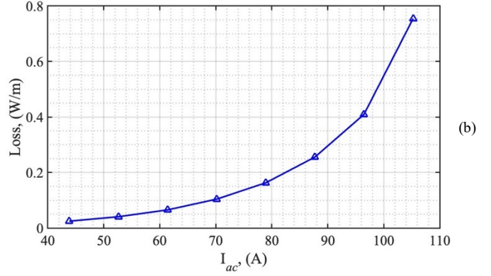
Fig. 9: Losses on the SCs by the 3D FEM and by the 2D single-slot model for two different tapes orientation (a), and zoom for the 2D \perp tapes (b).
