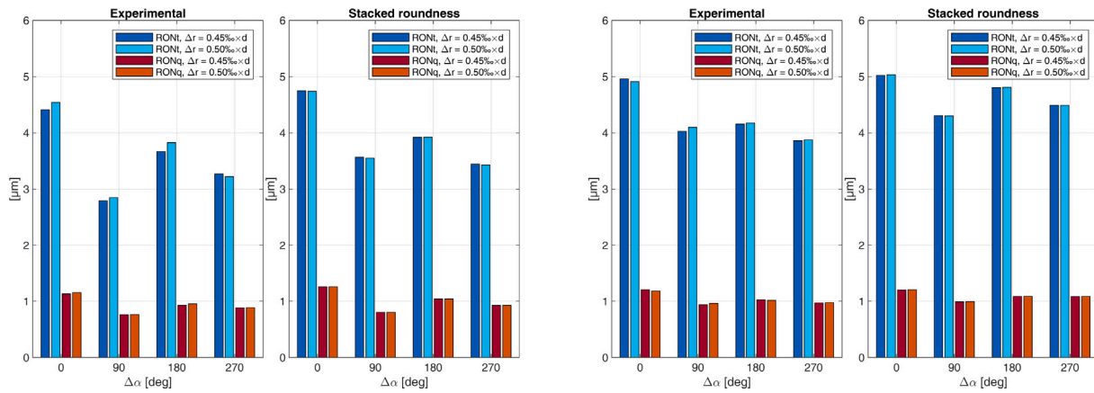
Fig. 17. Variation of the summed roundness RONt and RONq of the experimentally measured profile and the summed profile, as a function of the relative orientation \Delta\alpha , for 2 mounting conditions (in blue/red and light-blue/orange). The results are shown for the upper raceway mid-section (left) and lower raceway mid-section (right) measuring locations. \Delta r is the bearing radial internal clearance reduction in mounted condition and d is the bearing bore diameter.
