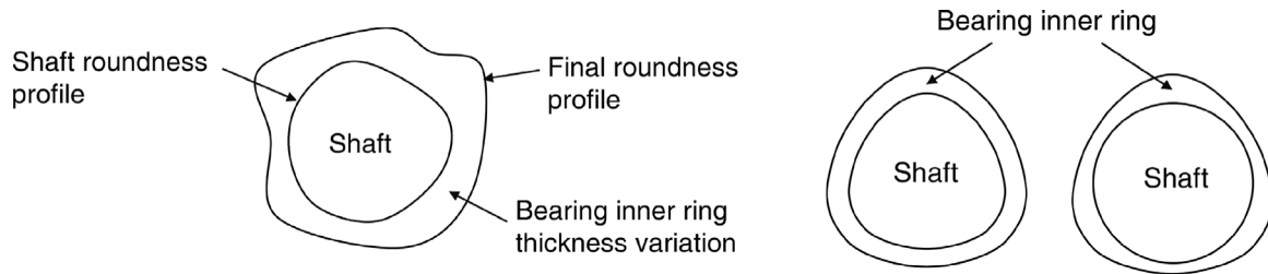
Fig. 2. Schematic representation of the final roundness profile of the IR due to the stacking of the shaft roundness error and the IR thickness variation (left). Schematic visualization of the roundness error formation of an installed bearing IR in two specific examples (right), modified from [2].
