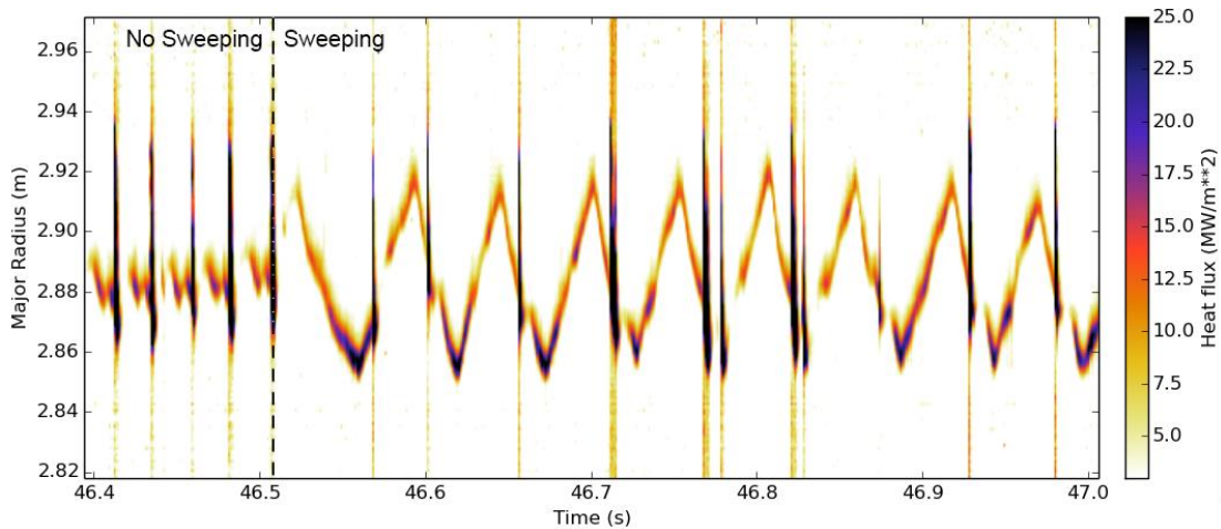
Figure 7: Heat flux on Tile 6 inferred from the IR camera temperatures, as a function of time and major radius, for a 20Hz sweeping test (#92324). Regular 42Hz ELMs are seen before the sweeping starts at 46.5s, after which the ELMs quickly synchronise with the sweeping.
