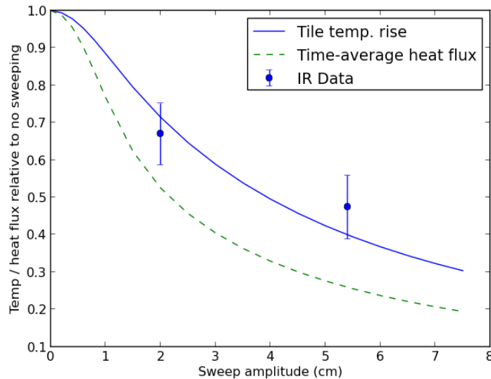
Figure 3: Modelled scaling of tile temperature rise (solid line) and heat flux (dashed line) at the sweep centre position, averaged over 1 sweep period with varying sweep amplitude after 2.5s of sweeping for a pulse similar to pulse 89297. Experimental points from pulses 89295 and 89296 are shown for comparison.
