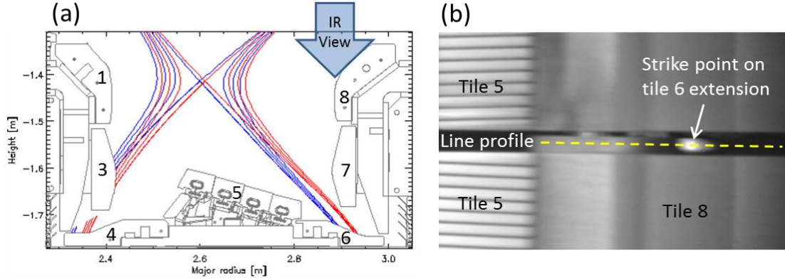
Figure 1: (a) Poloidal cross-section of the JET divertor showing magnetic flux contours at two different times during a pulse with sweeping. JET divertor tile designations are shown by the black numbers on the image and the IR camera viewing direction is indicated. (b) IR camera view of the outboard strike point on the tile 6 extension, showing the line profile used for tile temperature analysis (dashed line).
