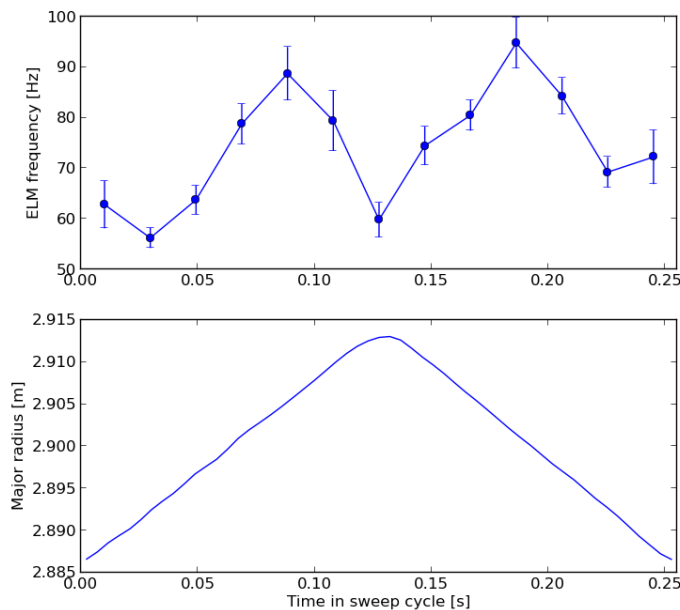
Figure 6: Variation of ELM frequency over the sweep cycle during JET pulse 90271 (3cm, 4Hz sweeping). Top: coherent average of the ELM frequency over 24 sweep cycles. Bottom: strike point major radius.
