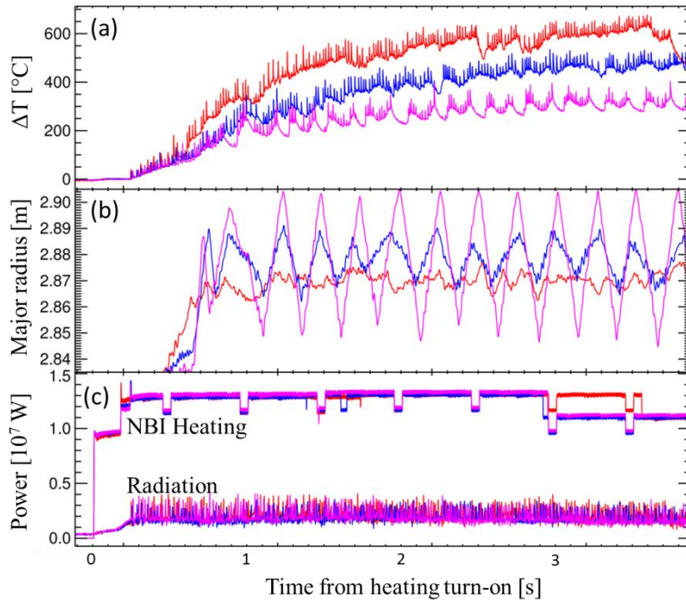
Figure 2: Comparison of pulses with different sweep amplitudes: no sweeping (#89297, red lines), 2cm sweeping (#89296, blue lines) and 5.4cm sweeping (#89295, pink lines). (a) Tile surface temperature rise at the strike point position / sweep centre (b) Strike point position / sweep centre (c) Input and radiated power.
