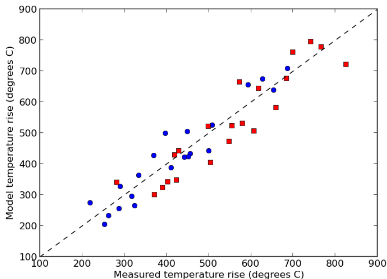
Figure 5: Comparison between measured and modelled tile temperature rise in sweeping pulses. Circles: minimum temperature during sweep cycle, squares: maximum during sweep cycle. The dashed line is y = x .
