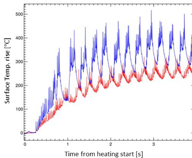
Figure 4: Comparison of measured surface temperature evolution on tile 6 at R = 2.86\text{m} (blue line) and R = 2.90\text{m} (red line) in JET pulse 89295 (pink lines in figure 2).
