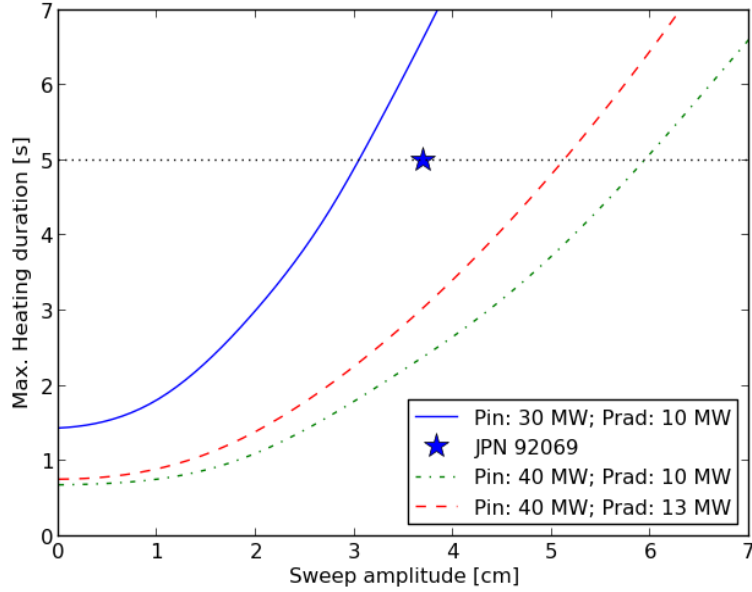
Figure 8: Estimated heating duration before reaching tile 6 temperature limits for I_p=2.4\text{MA} , B_T=2.8\text{T} hybrid plasmas with 4Hz sweeping. The three curves indicate the expected pulse length limit for different input power and radiation levels as indicated on the figure. The star represents the longest pulse with P_{in} = 30\text{MW} , P_{rad} = 10\text{MW} run during the recent campaigns (#92069). The horizontal dotted line is the desirable pulse length of 5s.
