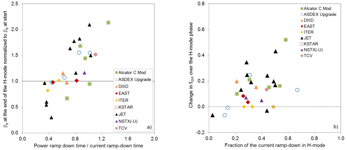
Figure 8: a) The change in \beta_p over the first part of the termination phase, up to the H-L back transition versus the ratio of power ramp-down time to current ramp-down time. b) The change in f_{GW} over the first part of the termination phase, up to the H-L back transition, versus of the fraction of the current ramp-down kept in H-mode. Note that the modelled ITER cases simply assume that f_{GW} remains constant.
