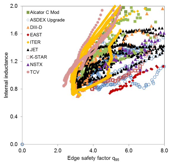
Figure 5: The traces of each entry in \ell - q space.
