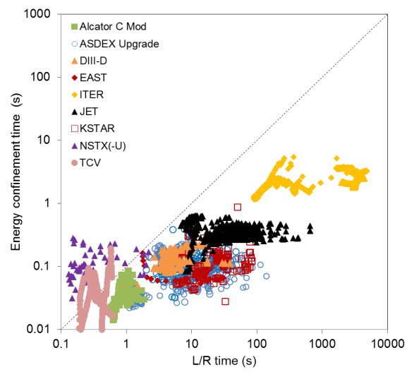
Figure. 3: The energy confinement time, \tau_E , versus the L/R time, \tau_{L/R} , for each time step during a number of database terminations in devices of different size.
