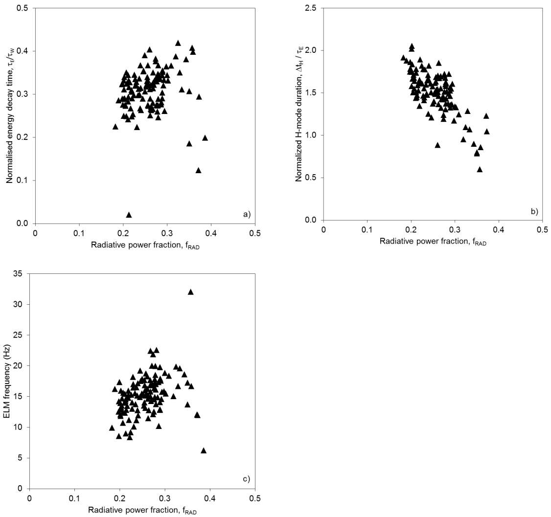
Figure 12: A series of 121 near identical discharges that were carried out at JET (JET Pulse numbers from 83623 to 83777). All operated in H-mode at I_p=2.0\text{MW} , q_{95}=3.4 with an auxiliary Neutral Beam (NB) heating of P_{\text{NB}}\sim 11\text{MW} . At the start of the current ramp-down, the auxiliary heating power was stepped down to zero, after which the plasma remains in H-mode for a time \Delta t_H . a) Shows the inverse ratio of the average energy decay time and the steady-state energy confinement time at the start of the termination, \tau_E/\tau_W . b) Shows \Delta t_H , normalized to the energy confinement time, \tau_E , as a function of the radiative power. c) Shows the ELM frequency versus the radiative power.
