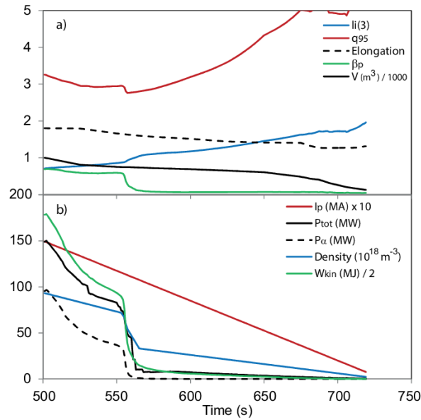
Figure 1: A modelled ITER termination (Corsica Hmode_15MA_13) from I_p=15\text{MA} at full performance ( W_{\text{kin}}=350\text{MJ} , P_\alpha=100\text{MW} ) taking approximately 220s. a) Shows the time traces of the internal inductance, \ell_i , the q_{95} , the elongation, \kappa , the poloidal \beta , and volume (in units of 1000\text{ m}^3 ). b) Shows the plasma current, I_p , in units of (in units of 100kA), the total input power, P_{\text{tot}} , the part from \alpha -heating, P_\alpha , the density (in 10^{18}\text{ m}^{-3} ) and the kinetic energy, W_{\text{kin}} . The H-L back transition is visible as fast drop in \beta_p and W_{\text{kin}} , around t=570\text{s} .
