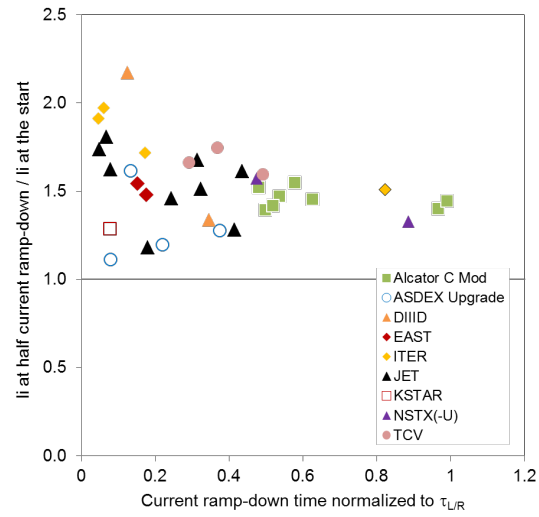
Figure 10: Existence diagram of the relative change in I_i over half the current ramp-down versus the ratio of the averaged current decay time and \tau_{L/R} .
