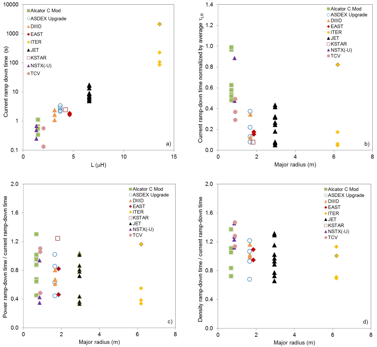
Figure 2: Existence diagrams of database entries showing a) the current ramp-down time versus the device inductance, L , b) the current ramp-down time normalized to \tau_{L/R} , versus major radius c) the relative power ramp-down time versus major radius. d) the relative density ramp-down versus major radius
